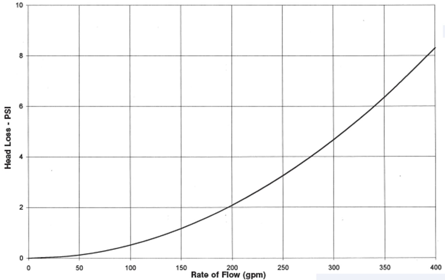
Head Loss: 3" Fire Hydrant Meter Performance Curves
